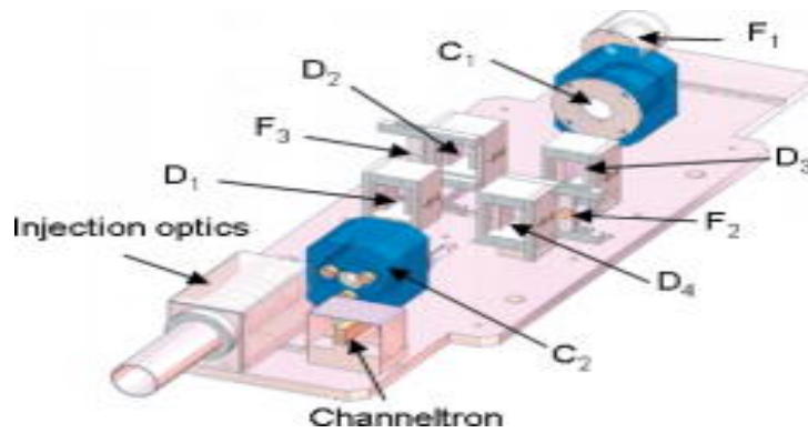
Figure 7. A three dimensional scale drawing of Mini-Ring. The ion optical elements—two conical mirrors and four deflector—are carefully positioned on a common mounting plate.
