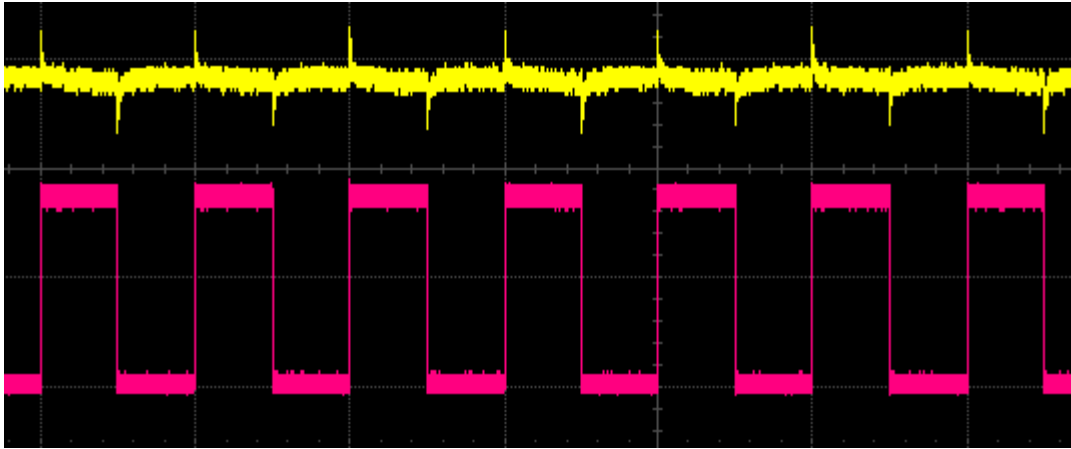
Figure 22. Charge detector signals (yellow) with negatively pulsed (pink) by waveform generator. The axis is 100 mV/div for charge detector signals, and 1V/div for the waveform generator pulse. The frequency is 5 kHz.
