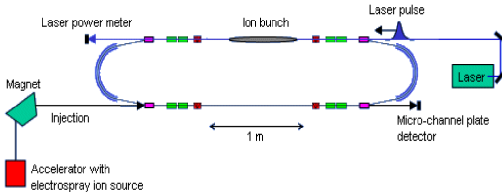
Figure 1. Schematic diagram of the electrostatic ion storage ring ELISA
