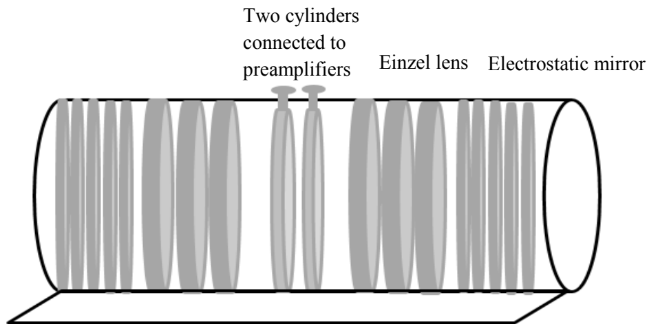
Figure 39. The new flexible EIBT with two cylinder image charge detectors.
