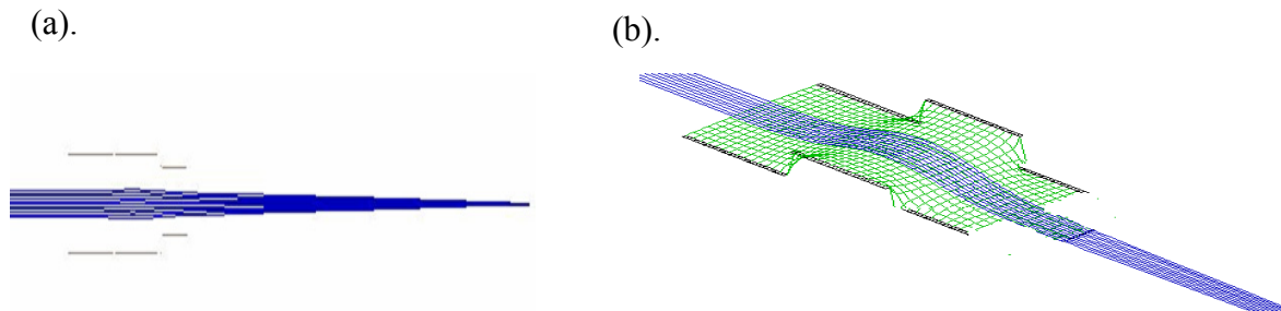
Figure 12. (a). An XY view of an Einzel Lens. A group of positive ions are flown into the lens at initial parallel trajectories and then bend to focal point. (b). The focusing effect is shown in the potential energy map.
